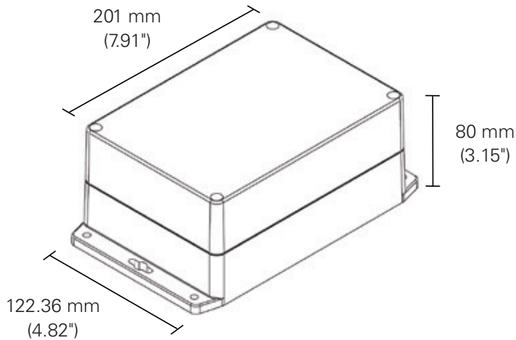
Figure106: iQ GATEway™ Battery Data Transmitter Dimensions
