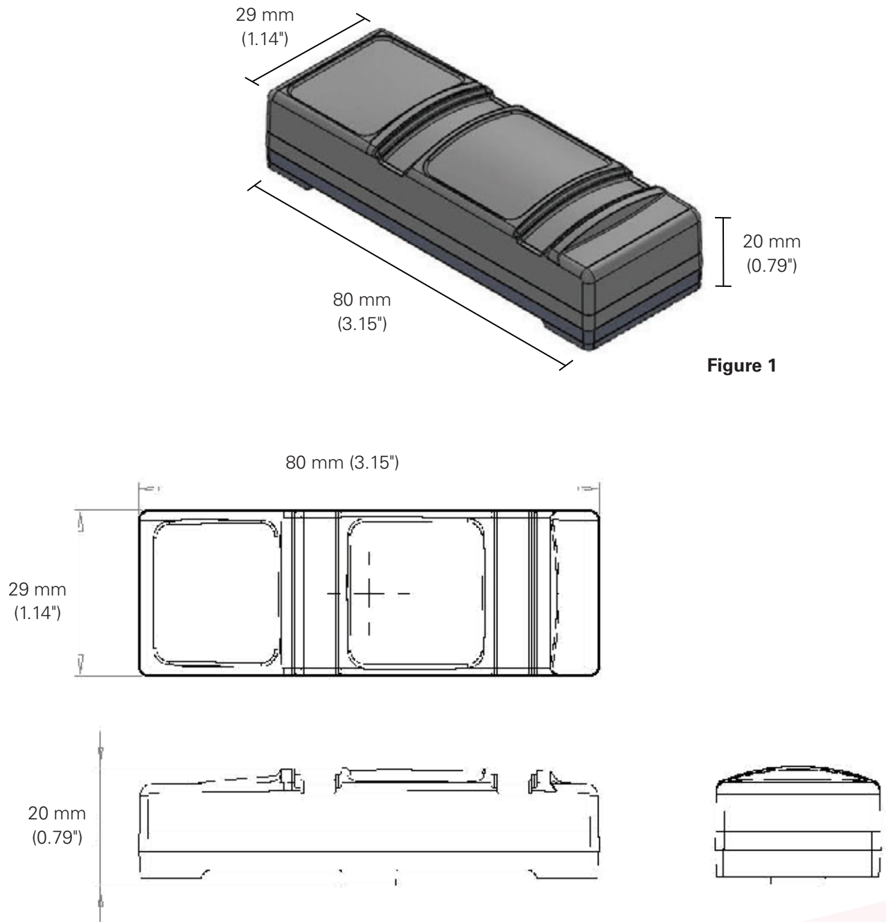
Figure 1: iQ Mini™ Battery Monitoring Device Dimensions
