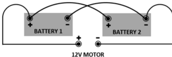
Battery Sketch 2
