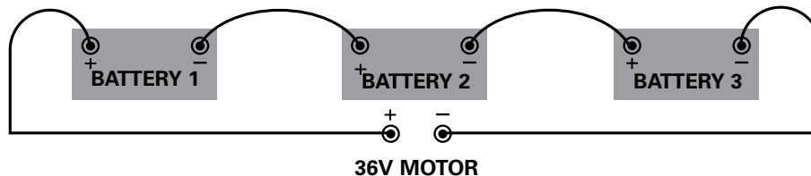
Battery Sketch 5
