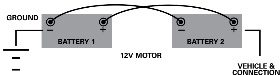
Battery Sketch 3
